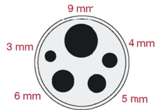
Multi-hole M01 (MTC-320 / 650 A)
